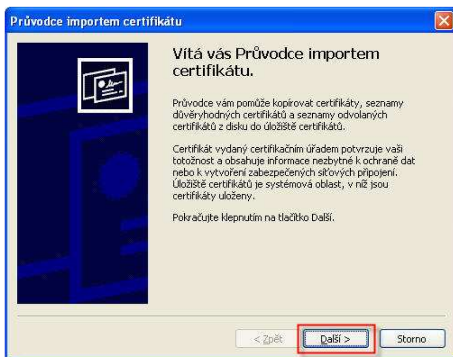
Windows XP
