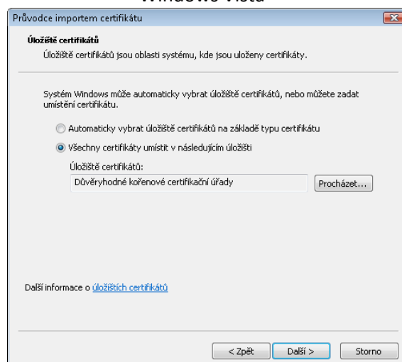
Windows Vista
