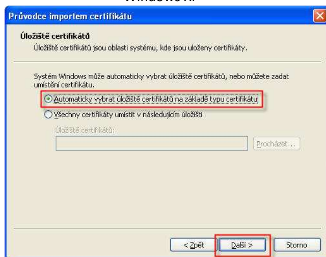
Windows XP
